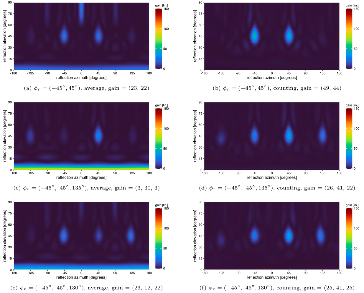
Fig. 8. Far field patterns after configuring the RIS for beam splitting. The RIS is configured for the reflection ( \theta_r = 45^\circ, \phi_r = 0^\circ, \theta_i = 0^\circ ). Reported gains are in linear scale. For comparison, the gain for the single beam case is 108.
