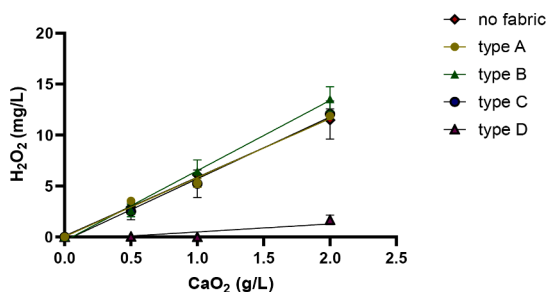
Fig. 5. Linear correlation between \text{H}_2\text{O}_2 yield at t = 24 h and \text{CaO}_2 granules' dose directly applied (no fabric) and applied enclosed in GEF types A–D.
