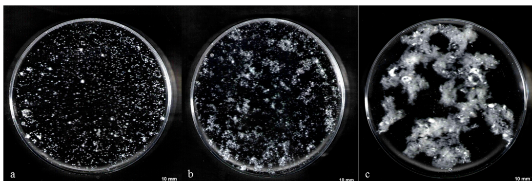
Figure 9. Images of (a) pelletized biomass, (b) dispersed mycelia using commercial nitrogen sources, and (c) dispersed mycelia using 200 mg/L FAN of soybean cake hydrolysate as nitrogen sources. Images were taken at 48 h of submerged fermentation of R. arrhizus NRRL 2582 using 25 g/L of initial glucose and 0.2 g/L initial ammonium sulphate concentration.
