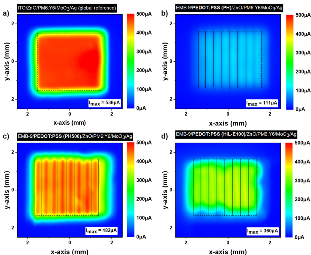
Figure 3. Photocurrent mapping images of 9 \text{ mm}^2 inverted OPV devices: (a) ITO-based reference device and ITO-free devices using the EMB nine-line Ag np grid with different PEDOT:PSS formulations, (b) PH, (c) PH500, and (d) HIL-E100. The reference device in that case was ITO/ZnO/PM6:Y6/MoO 3 /Ag.
