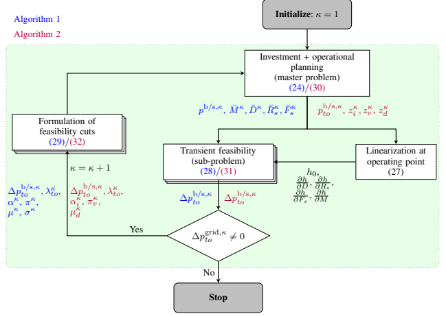
Fig. 1: The proposed decomposition algorithms for the inertia-aware MG planning problem where variables are differentiated with A1 (blue), A2 (purple), and both A1 and A2 (black).
