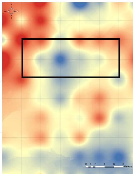
Figure 17. Difference values as calculated for OSAVI index
