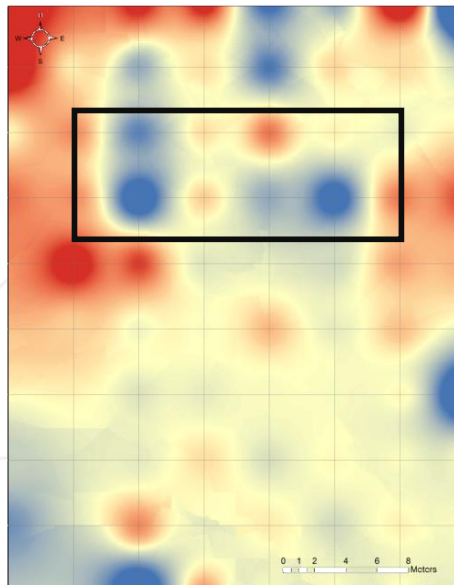
Figure 25. Difference values as calculated for ARVI index
