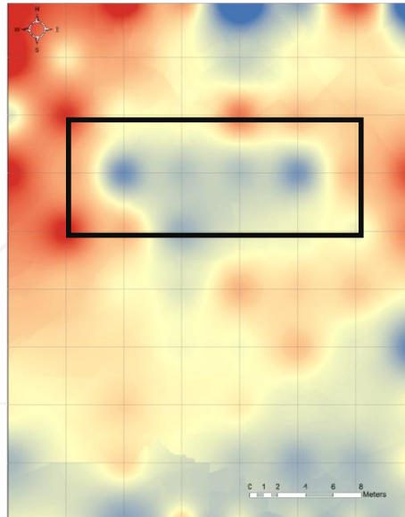
Figure 24. Difference values as calculated for DVI index
