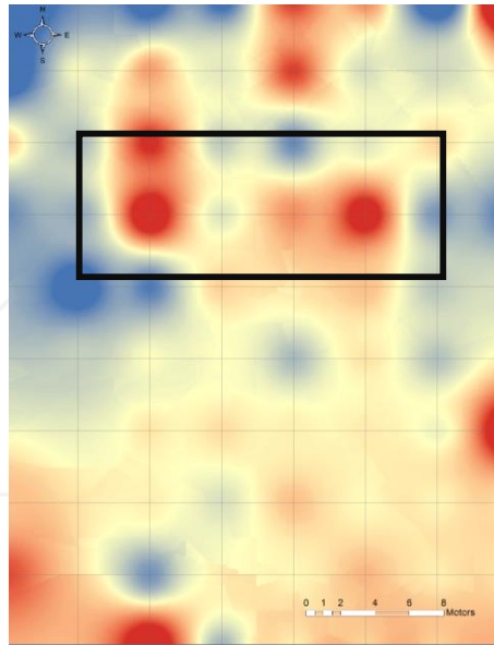
Figure 16. Difference values as calculated for RVI index
