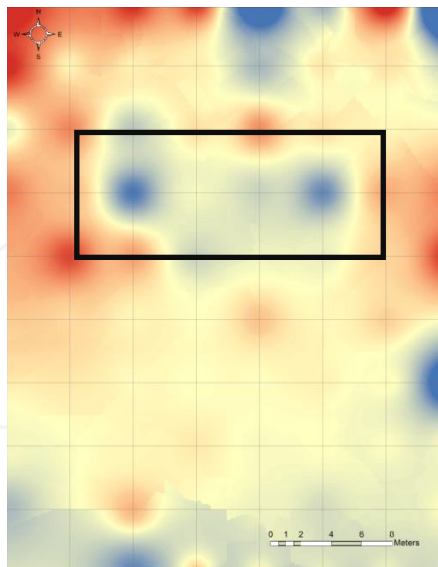
Figure 13. Difference values as calculated for SRxNDVI index
