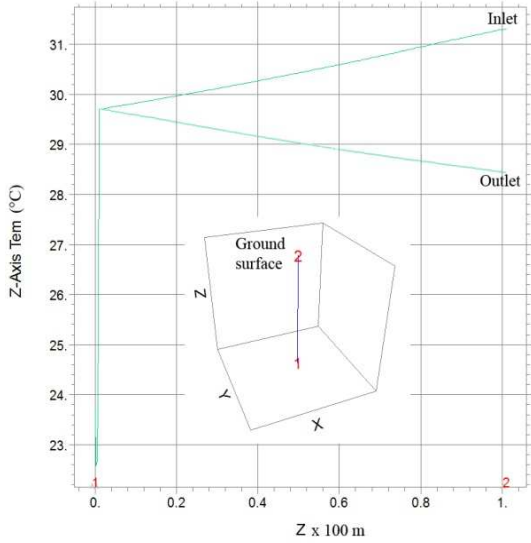
Fig. 6 Vertical temperature profile of the fluid in the heat exchanger (1-bottom, 2-surface) after 9.3 hours of operation
