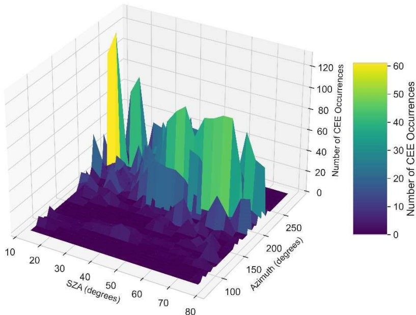
Figure 5: Three-Dimensional distribution of CEE frequencies as a function of solar zenith and azimuth angles.
