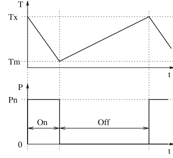
Fig. 20. Temperature and power cycles of a typical refrigerator.
