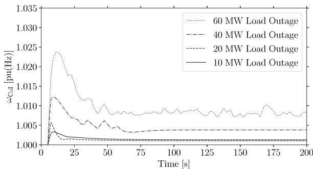
Fig. 24. Clusterized frequency load control combined with ESSs [148].
