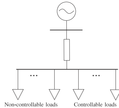
Fig. 17. Two-bus system used in simulations. Two groups of devices, non-controllable and controllable devices, are connected to the second bus, which is connected to a swing bus via a transmission line.
