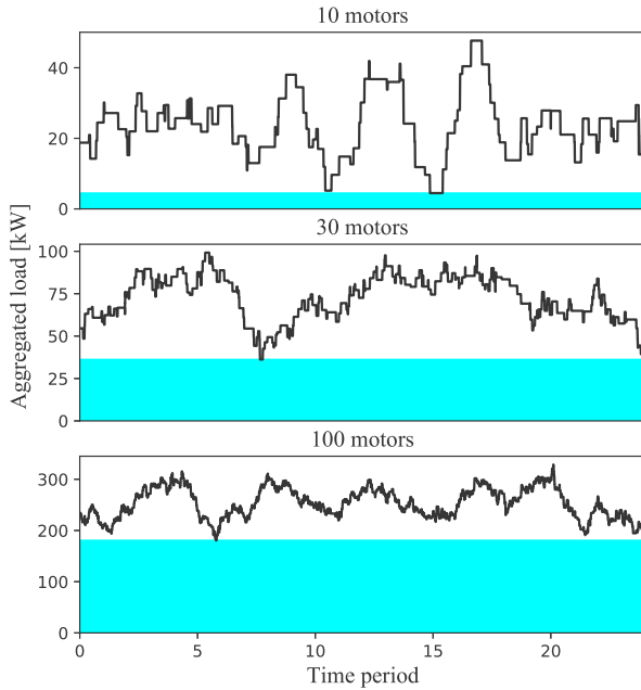
Fig. 15. Three different groups with aggregated loads under stochastic behavior. The devices have an average of 5 kW size, and size, duty-cycle, activation time and periodicity are randomly assigned according to normal distributions. The top panel demonstrates a situation where aggregation of ten motors provides less than 20% of the average power for continuous flexibility reserve. The middle panel shows an improved performance, with over 45% available flexibility. The bottom panel represents a higher flexibility available at any given time, with over 70% of the average load being available at any given time. The time periods are agnostic (i.e., may be applied to second-, minute- or hourly-level intervals).
