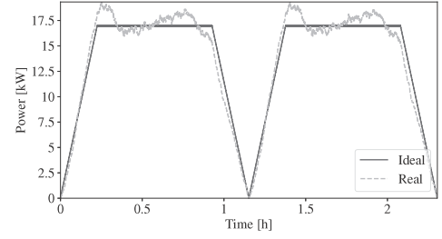
Fig. 21. Total active power consumption of 1000 refrigerators with d = 19.21\% .
