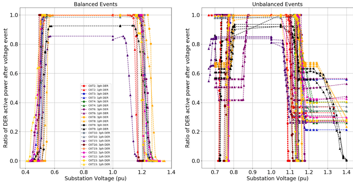
Fig. 9. Trip profile of distributed energy resources across multiple feeders with 100% distributed energy resource penetration with respect to load [108].
