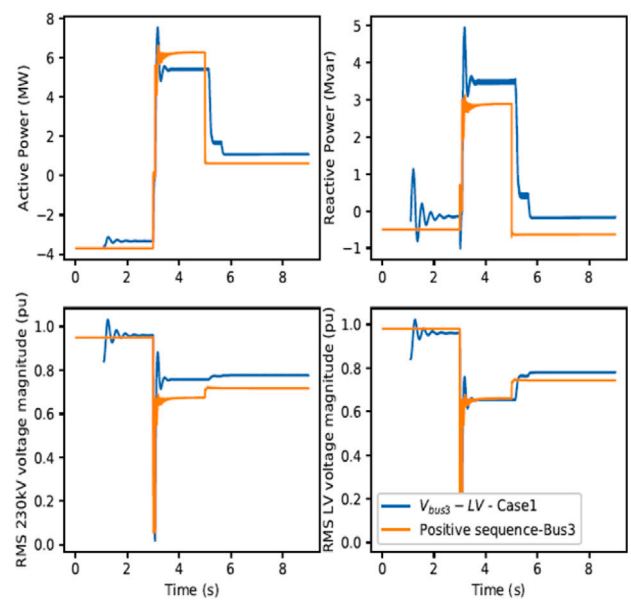
Fig. 11. For a transmission system fault, comparison of response from equivalent DN model at a transmission bus (orange curve) with the response from a detailed distribution feeder model connected at the same transmission bus (blue curve) [111].
