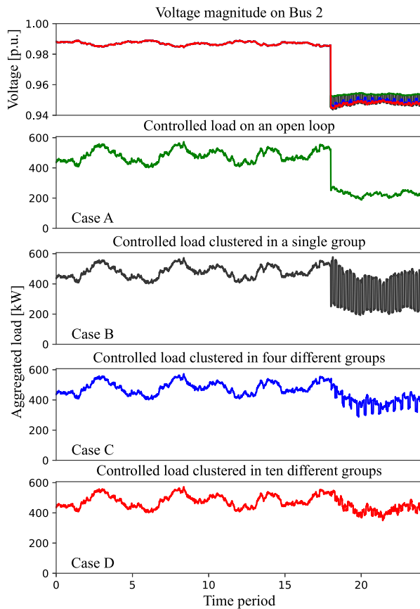
Fig. 18. A single plot of four cases' voltages (top panel) and each of their aggregated load responses (lower four panels). A fault located in the swing bus leads to the second bus to dip below the minimum 0.95 pu limit, which triggers controllable loads (half of the aggregated devices' load). Case A denotes the open-loop case, where controllable loads are not turned on again even after the voltage recovers above the minimum limit; Case B depicts a closed-loop response where all controllable loads act in the same time, leading to an oscillatory behavior; and Cases C and D demonstrate how aggregating devices in smaller clusters and introducing a delay for their activation reduces the oscillatory behavior witnessed in Case B. The time periods for the simulation are agnostic (i.e., may be applied to second-, minute- or hourly-level intervals).
