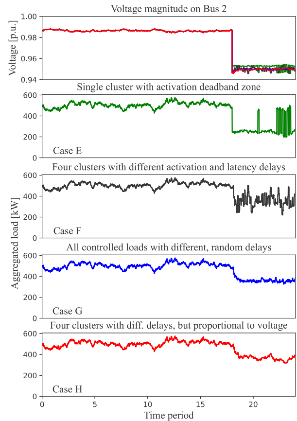
Fig. 19. A single plot of four cases' voltages (top panel) and each of their aggregated load responses (lower four panels). A fault located in the swing bus leads to the second bus to dip below the minimum 0.95 pu limit, which triggers controllable loads (half of the aggregated devices' load). Case E depicts the results for the same settings as Case B, but introducing a dead-band zone during which the loads are not turned back on. While it is more smooth than Case B, it is still prone for some periods with oscillatory behavior. Case F showcases the results for the same settings as Case C, but using different time delays for the activation of different groups, in which it is clearly visible that the devices respond in a very unstable manner. Case G assumes all controllable devices have different delays in activation or latency, which leads to a very smooth system-wide response, even if some minority of the loads might be activated too often. Finally, Case H depicts the results for a simulation with the same settings than Case F, but introducing a coordination scheme where some of the devices in each cluster are turned off, proportional to the local voltage. It depicts another very smooth response, but is the case that requires the most coordination among all cases showcased here. The time periods for the simulation are agnostic (i.e., may be applied to second-, minute- or hourly-level intervals).
