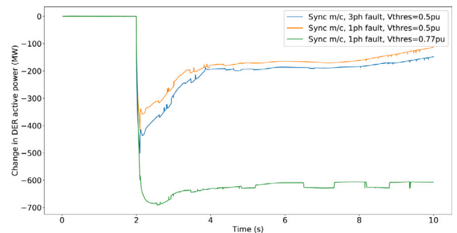
Fig. 10. DER impact on bulk power system fault behavior [113].
