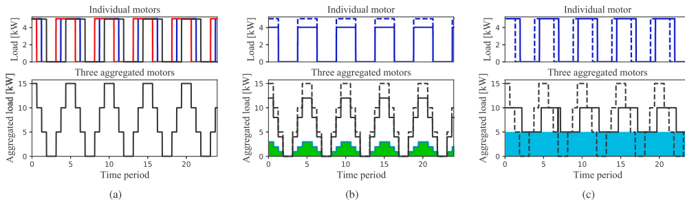
Fig. 14. Three applications with 5 kW aggregated in (a) a basic operation, (b) a power shift of 20% enabling a varying flexibility reserve across selected intervals, and (c) a time shift across all applications enabling a continuous flexibility reserve of 5 kW.
