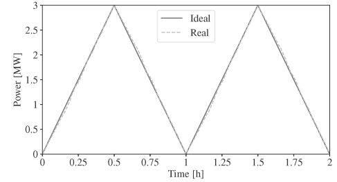
Fig. 22. Total active power consumption of 1000 heat pumps with d = 50\% .
