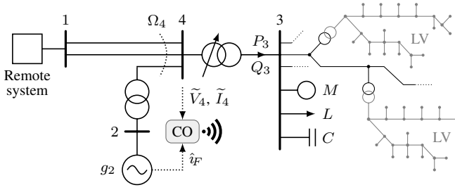
Fig. 8. Test system with explicit modeling of HV, MV, and LV networks. The coordinator (CO) sends signals to DERs and FLs.
