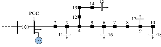
Fig. 2. Modified CIGRE European low voltage network.
