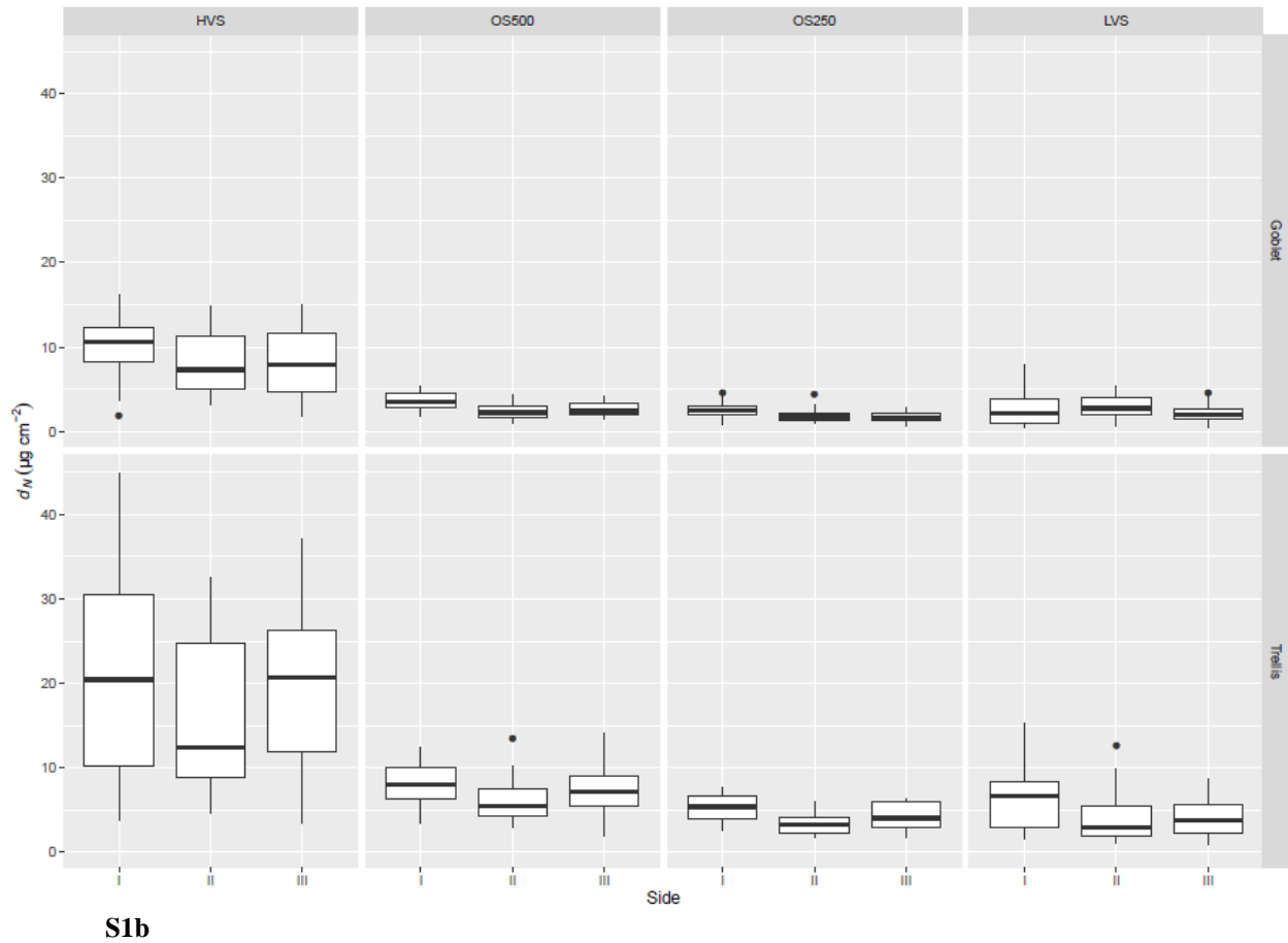
Figure S1: Normalized deposition ( d_N ) on (a) different heights of vines (A - lower – see Fig. 3 for details) and (b) different sides (II - interior part of the vine) for the goblet and the trellis training systems. Boxplots show the median for each treatment, box boundaries show the 25th and 50th percentile, while whiskers extend to 1.5 times the interquartile range (IQR). Points beyond 1.5 times the IQR are plotted individually. See text for results of statistical analyses.
