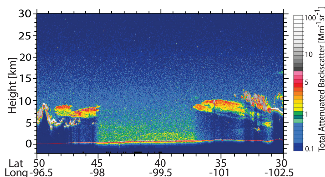
Figure 14. CALIPSO lidar observations of tropospheric smoke over North and South Dakota (45–48.5° N, 7–9 km height) and over Texas (33–37° N, 8–10 km height) on 13 September 2020, around 9:15 UTC (CALIPSO, 2020a). The smoke layers (in yellow to red) originated from British Columbia (North and South Dakota plume, travel time of 24 h) and from California (Texas plume, 2–5 d of travel time) as HYSPLIT backward trajectories indicate (HYSPLIT, 2020).
