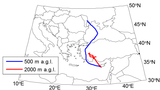
Figure 12. Back trajectories of 96h arriving at Limassol on 20 May 2017 at 21:00 UTC.
