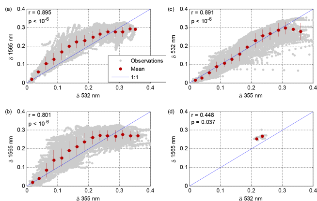
Figure 15. Comparison of particle linear depolarization ratio at different wavelengths. Observations represent 30 m vertical resolution and have been smoothed by a 300 m running mean. To reduce scatter, a stricter uncertainty threshold is applied, and only data for \sigma_{\delta} < 0.01 (at the 1565 nm wavelength) are included. The mean is calculated at intervals of 0.025 on the x axis, and error bars indicate standard deviation. (a) Depolarization ratio at 1565 nm (Halo) vs. depolarization ratio at 532 nm (PollyXT) at Limassol. (b) Depolarization ratio at 1565 nm vs. depolarization ratio at 355 nm (PollyXT) at Limassol. (c) Depolarization ratio at 532 nm vs. depolarization ratio at 355 nm at Limassol. (d) Depolarization ratio at 1565 nm vs. depolarization ratio at 532 nm at Vehmasmäki.
