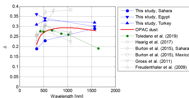
Figure 17. Particle linear depolarization ratio as a function of wavelength for dust observations in Table 2. Additionally, spectral dependency modelled with MOPSMAP based on the OPAC database for desert dust (Koepke et al., 2015; Gasteiger and Wiegner, 2018) and AERONET inversion by Toledano et al. (2019) are included.
