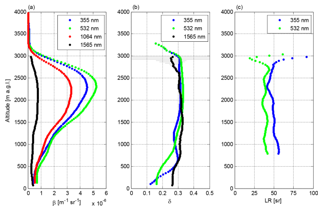
Figure 8. Averaged profiles at Limassol on 27 April 2017 at 19:00–20:00 UTC. All profiles have been smoothed by a 300 m running mean. (a) Backscatter by PollyXT (wavelengths 355–1064 nm) and attenuated backscatter by Halo (1565 nm). (b) Particle linear depolarization ratio. Error bars represent measurement uncertainty. (c) Lidar ratio. For PollyXT \beta_{355} and \beta_{532} , a near-range telescope is used for data < 900 m a.g.l.
