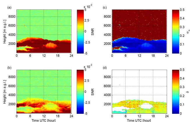
Figure 7. Limassol 27 April 2017 measurements with Halo Doppler lidar. (a) Time series of co-polar SNR at 300 s integration time. (b) Time series of cross-polar SNR at 300 s integration time. (c) Uncertainty in the depolarization ratio. (d) Particle linear depolarization ratio filtered with \sigma_\delta < 0.05 .
