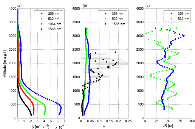
Figure 11. Averaged profiles at Limassol on 20 May 2017 at 19:55–21:30 UTC. All profiles have been smoothed by a 300 m running mean. (a) Backscatter by PollyXT (wavelengths 355–1064 nm) and attenuated backscatter by Halo (1565 nm). (b) Particle linear depolarization ratio. Error bars represent measurement uncertainty. (c) Lidar ratio. For PollyXT \beta_{355} , \beta_{532} , LR_{355} and LR_{532} , a near-range telescope is used for data <900 m a.g.l.
