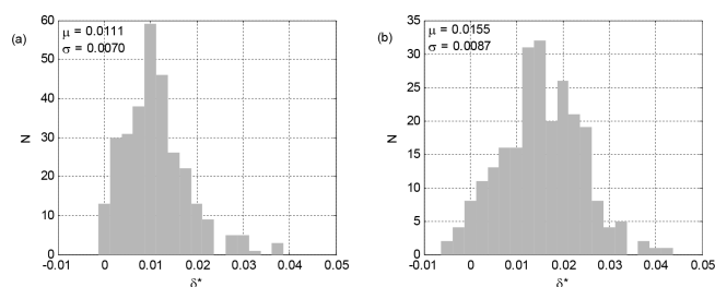
Figure 3. Ratio of cross-polar SNR to co-polar SNR at liquid cloud base measured with Halo Doppler lidar. (a) Distribution of cloud base \delta^* at Limassol. (b) Distribution of cloud base \delta^* at Vehmasmäki.
