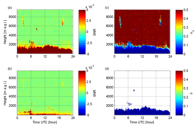
Figure 10. Limassol 20 May 2017 measurements with Halo Doppler lidar. (a) Time series of co-polar SNR at 300 s integration time. (b) Time series of cross-polar SNR at 300 s integration time. (c) Uncertainty in the depolarization ratio. (d) Particle linear depolarization ratio filtered with \sigma_\delta < 0.05 .
