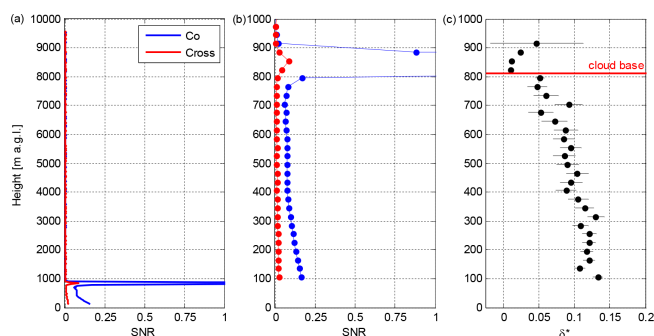
Figure 2. Profiles at Limassol, Cyprus, on 2 May 2017 at 12:08 UTC. (a) Co- and cross-polar SNR. A liquid cloud at approx. 800 m a.g.l. results in full attenuation of signal. Below cloud layer aerosol signal is visible. Above 1 km variability in SNR is due to instrumental noise only. (b) The same as panel (a) but limited to lowest 1 km a.g.l. (c) Ratio of cross-polar SNR to co-polar SNR up to 1 km a.g.l. calculated from profiles in panel (a). Error bars represent uncertainty due to instrumental noise estimated from SNR at > 1 km a.g.l. in panel (a).
