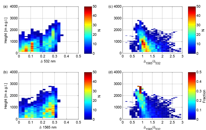
Figure 16. 2D histograms of the particle linear depolarization ratio and height at Limassol using 30 m vertical resolution smoothed by a 300 m running mean. Only data for \sigma_\delta < 0.01 (at the 1565 nm wavelength) are included. (a) Depolarization ratio at 532 nm. (b) Depolarization ratio at 1565 nm. (c) Ratio of depolarization ratios at 1565 and 532 nm. (d) Same as panel (c) but scaled with number of observations at each height.
