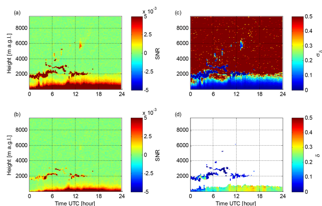
Figure 13. Vehmassmäki 15 May 2016 measurements with Halo Doppler lidar. (a) Time series of co-polar SNR at 350 s integration time. (b) Time series of cross-polar SNR at 350 s integration time. (c) Uncertainty in the depolarization ratio. (d) Particle linear depolarization ratio filtered with \sigma_{\delta} < 0.05 .
