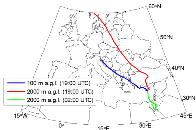
Figure 9. Back trajectories of 96 h arriving at Limassol on 27 April. Back trajectories arriving at 19:00 and 02:00 UTC are included.
