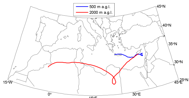
Figure 6. Back trajectories of 96 h arriving at Limassol on 21 April 2017 at 21:00 UTC.
