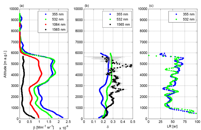
Figure 5. Averaged profiles at Limassol on 21 April 2017 at 20:00–21:30 UTC. All profiles have been smoothed by a 300 m running mean. (a) Backscatter by PollyXT (wavelengths 355–1064 nm) and attenuated backscatter by Halo (1565 nm). (b) Particle linear depolarization ratio. Error bars represent measurement uncertainty. (c) Lidar ratio. For PollyXT \beta_{355} , \beta_{532} , LR_{355} and LR_{532} , a near-range telescope is used for data < 900 m a.g.l.
