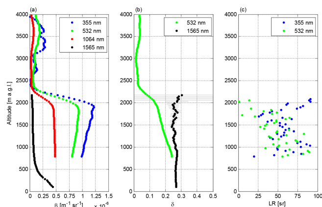
Figure 14. Averaged profiles at Vehmassmäki on 15 May 2016 at 19:00–21:00 UTC. All profiles have been smoothed by a 300 m running mean. (a) Backscatter by PollyXT (wavelengths 355–1064 nm) and attenuated backscatter by Halo (1565 nm). (b) Particle linear depolarization ratio. Error bars represent measurement uncertainty. (c) Lidar ratio.
