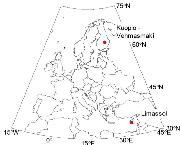
Figure 1. Locations of Vehmasmäki and Limassol measurement sites.
