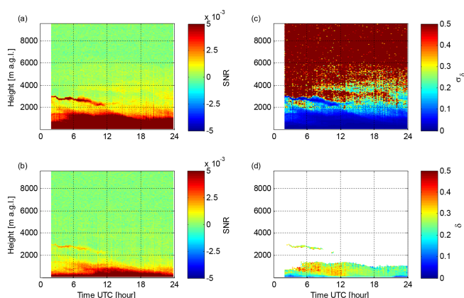
Figure 4. Limassol 21 April 2017 measurements with Halo Doppler lidar. (a) Time series of co-polar SNR at 300 s integration time. (b) Time series of cross-polar SNR at 300 s integration time. (c) Uncertainty in the depolarization ratio. (d) Particle linear depolarization ratio filtered with \sigma_\delta < 0.05 .
