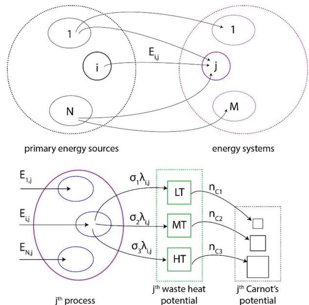
Fig. 2 Calculation methodology for WHR potential estimation
