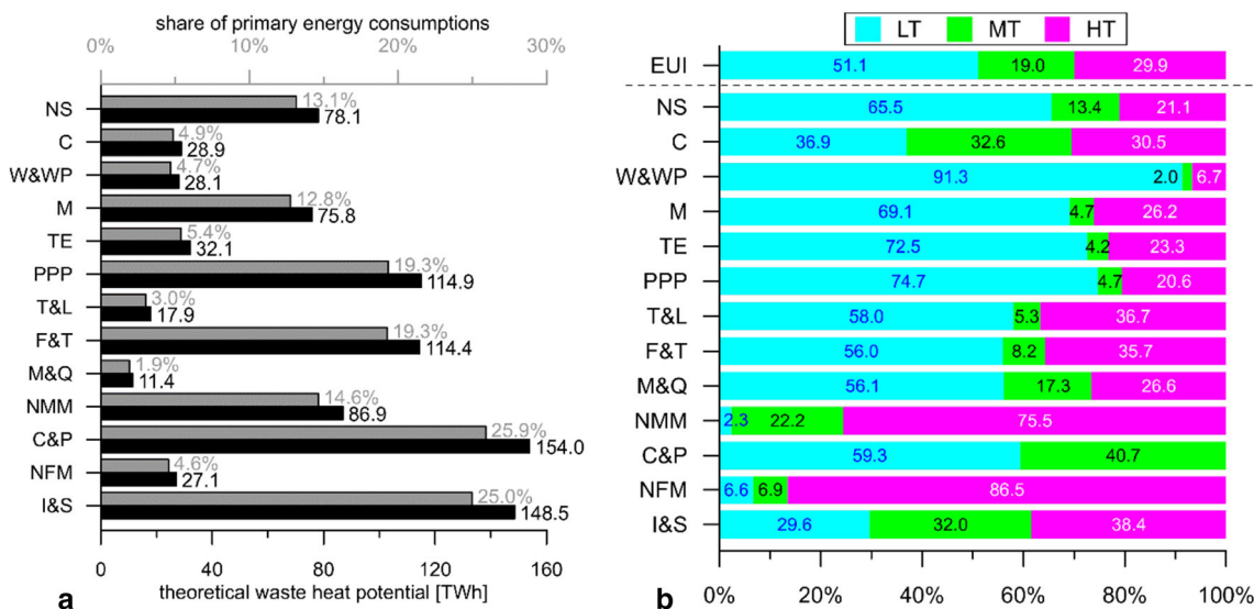
Fig. 6 a Theoretical WHR potential and relevance on primary energy consumptions for the EU industry, b breakdown of the theoretical WHR potential in the EU industry with respect to temperature levels
