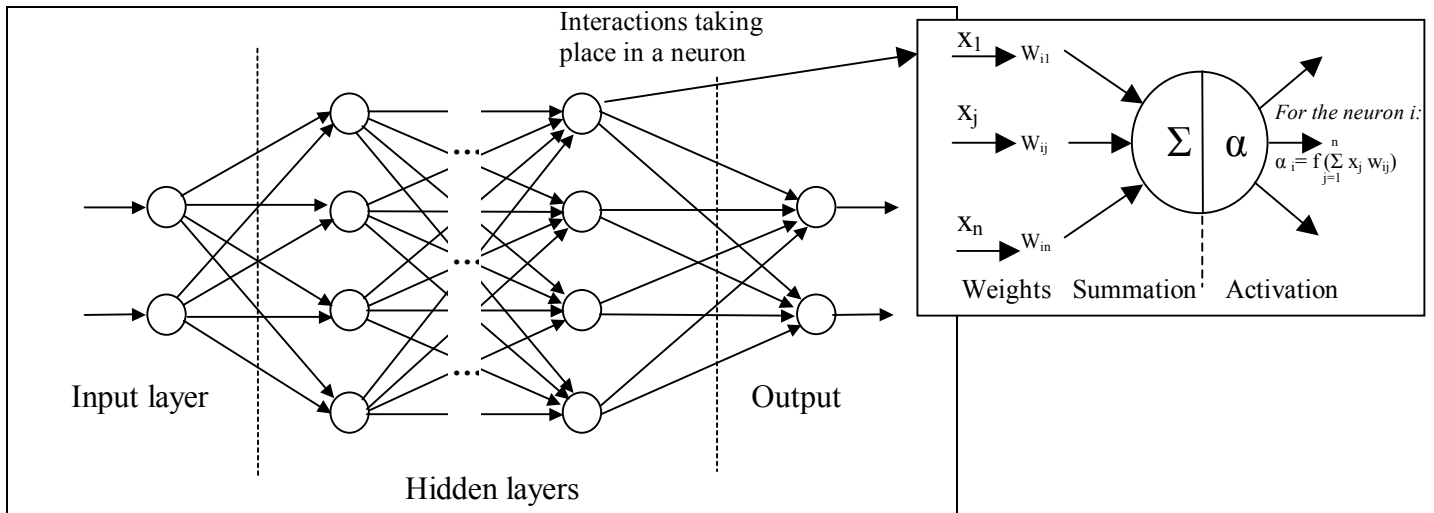
Figure 1: Schematic diagram of a multilayer feed forward neural network.
