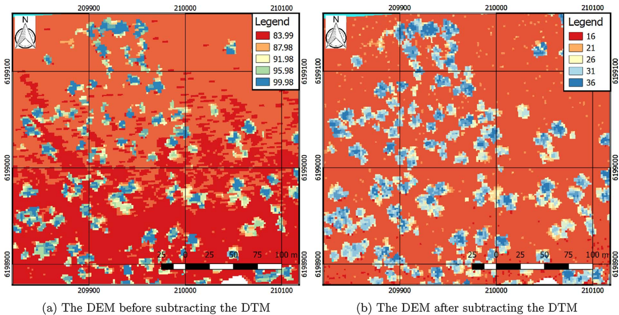
Fig. 5. The difference of the DEM before and after subtracting the DTM.
