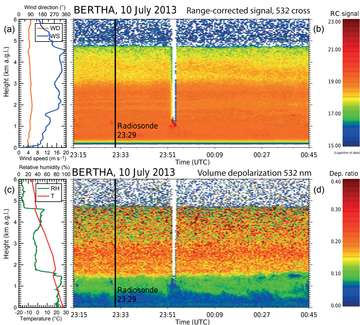
Figure 2. Saharan air layer (from 1.5 to 4.7 km height above ground level) above the marine boundary layer. Panel (b) shows the range-corrected cross-polarized 532 nm backscatter signal with temporal and vertical resolutions of 30 s and 7.5 m, respectively. Panel (d) shows the 532 nm volume linear depolarization ratio. The lidar observation was performed on 10 July 2013, 19:15–20:45 LT. A radiosonde was launched at 19:29 LT (indicated by black vertical lines). The radiosonde profiles of wind speed (WS) and wind direction (WD) are shown in panel (a), the profiles of relative humidity (RH) and temperature ( T ) in panel (c).
