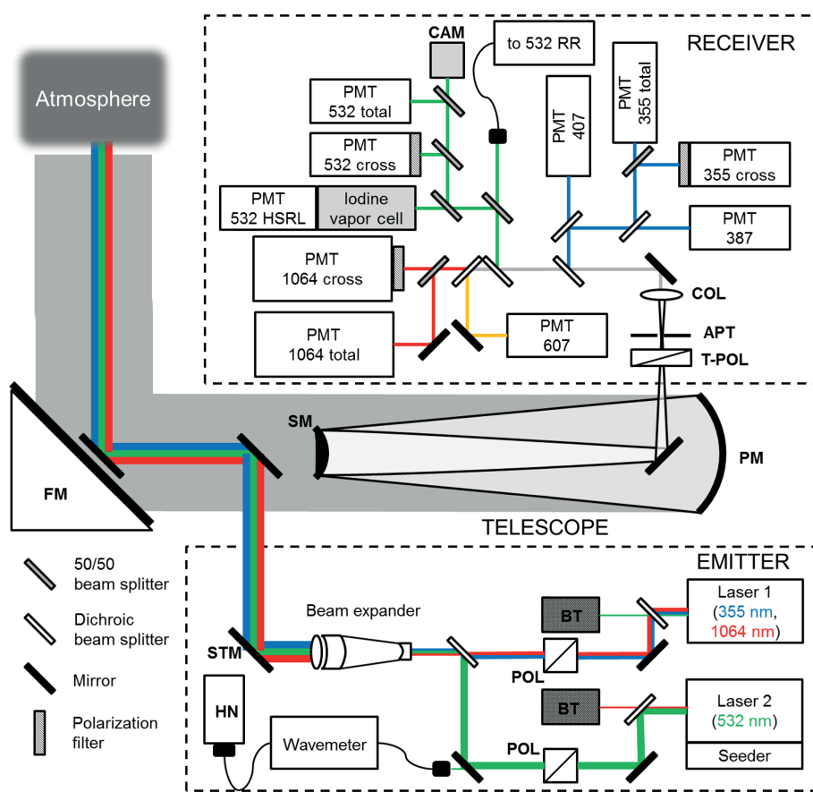
Figure 1. Sketch of BERTHA's emitter and receiver. All detection channels are photomultiplier tubes (PMTs, operated in the photon counting mode) and the numbers indicate the central wavelength of transmission in nanometers of the interference filter. Polarization filters are oriented perpendicular to the emitted state of polarization and are placed in front of the “cross” channels. The “total” channels measure the cross and the parallel part of the backscattered light. POL denotes polarizer to purify the laser polarization, BT denotes beam trap, HN denotes helium neon laser as reference for the wavemeter, STM denotes steering mirror with stepper motors to adjust the overlap, CAM denotes camera to visualize the overlap, FM denotes flat mirror (consisting of two mirrors, the small one for emitted pulses, the large one for backscattered light), PM stands for main or primary mirror and SM for counter or secondary mirror of the Cassegrain telescope, and TPOL means turnable polarization filter for \Delta 90^\circ calibration, APT motorized aperture, and COL collimator. Finally RR denotes rotational Raman channel, and HSRL denotes the high-spectral-resolution lidar channel.
