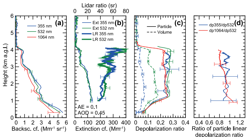
Figure 9. 3 h mean profiles of (a) the particle backscatter coefficient at three wavelengths, (b) the extinction coefficient and lidar ratio at two wavelengths, (c) the volume and particle linear depolarization ratio at three wavelengths, and (d) the ratio of the 355 to 532 nm and 1064 to 532 nm particle depolarization ratio. The lidar observation was performed on 20–21 June 2014, 23:10–02:10 UTC. The vertical signal smoothing window length is 200 m (backscatter coefficient, depolarization ratio) and 750 m (extinction coefficient, lidar ratio). Error bars indicate the retrieval uncertainty.
