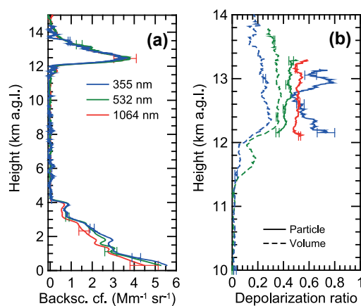
Figure 6. (a) Aerosol layers below 4 km height and cirrus layer from 12 to 14 km height in terms of particle backscatter coefficient at three wavelengths observed with BERTHA on 20–21 June 2014, 23:10–02:10 UTC (signal averaging period), and (b) cirrus ice crystal depolarization ratio (solid lines, volume depolarization ratio as dashed lines) at three wavelengths. At 1064 nm the volume depolarization ratio is equal to the particle depolarization ratio. The vertical signal smoothing length is 200 m. Error bars show the relative uncertainty in the retrievals (1 standard deviation).
