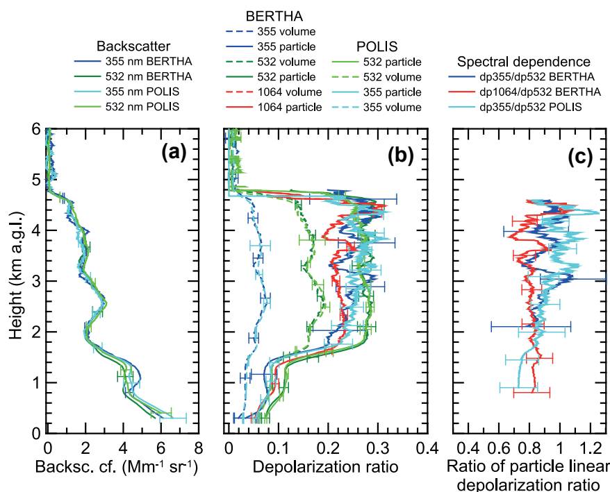
Figure 5. Comparison of POLIS and BERTHA depolarization-ratio observations. Shown are 45 min mean profiles of (a) the particle backscatter coefficient at 355 (POLIS light blue, BERTHA dark blue) and 532 nm wavelength (POLIS light green, BERTHA dark green); (b) the volume (dashed curves) and particle linear depolarization ratio (solid lines) at 355 nm (POLIS light blue, BERTHA dark blue), 532 nm (POLIS light green, BERTHA dark green), and 1064 nm (BERTHA, red line, equal volume and particle depolarization-ratio profiles); and (c) the ratio of the 355 to 532 nm particle depolarization ratio (POLIS light blue, BERTHA dark blue) and 1064 to 532 nm particle depolarization ratio (BERTHA, red). POLIS and BERTHA observations were taken simultaneously on 11 July 2013, 00:00–00:45 UTC. Error bars indicate the retrieval uncertainty (1 standard deviation). The vertical signal smoothing window length is 200 m (BERTHA, POLIS).
