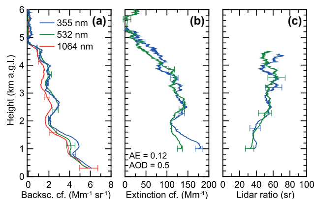
Figure 4. 45 min mean profiles of (a) the particle backscatter coefficient at three wavelengths, (b) extinction coefficient at two wavelengths, and (c) extinction-to-backscatter ratio (lidar ratio) at two wavelengths, measured with BERTHA on 11 July 2013, 00:00–00:45 UTC. Error bars indicate the retrieval uncertainty (1 standard deviation). The vertical signal smoothing window length is 200 m (backscatter coefficient) and 1000 m (extinction coefficient, lidar ratio). The column values of the Ångström exponent (AE 440–870 nm) and the aerosol optical depth (AOD) from the closest AERONET observation are indicated.
