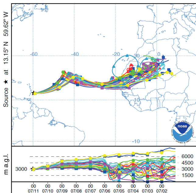
Figure 3. Ensemble of 10-day backward trajectories (Stein et al., 2015; HYSPLIT, 2016) for 11 July 2013, 01:00 UTC, arriving at 3000 m over Barbados.
