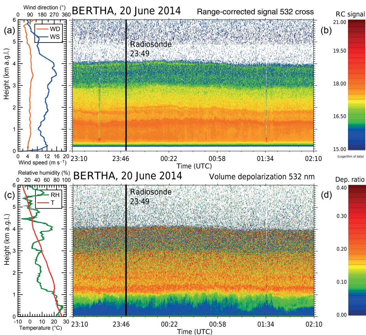
Figure 7. Saharan air layer (from 1 to 4 km height) above the marine boundary layer. The same parameters as in Fig. 2 are shown. The lidar observation was performed on 20 June 2014, 19:10–22:10 LT. The radiosonde was launched at 19:49 LT (indicated by black vertical lines).
