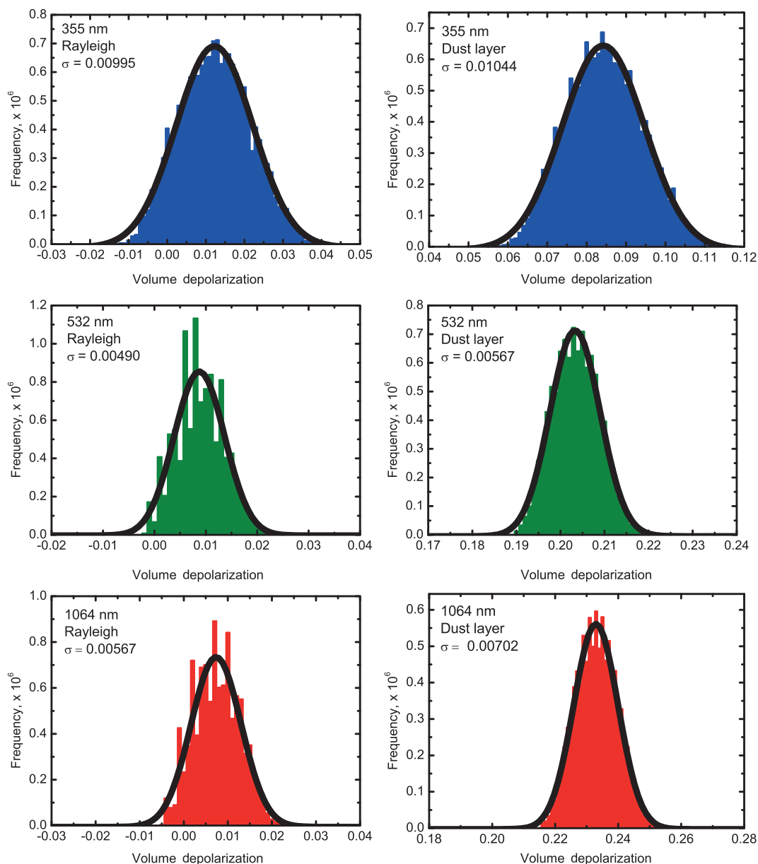
Figure A1. Frequency distribution (in millions of individual computations) of the volume depolarization ratio derived by a Monte Carlo simulation of the system parameters of the BERTHA lidar system (Table A1) within their uncertainties. For each wavelength the Rayleigh depolarization and a typical value in the dust layer was chosen as the input value (true value), given in Table A2. The standard deviation \sigma of the Gaussian fit (black line) is given to estimate the error of the volume depolarization ratio.
