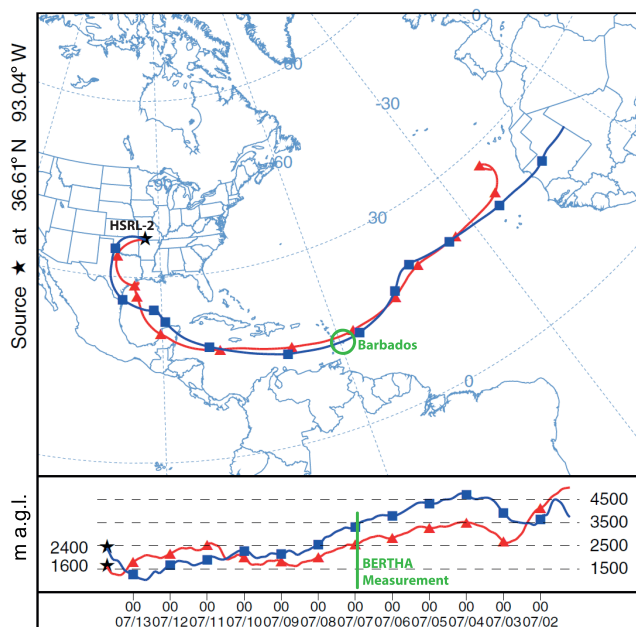
Figure 10. 12.5-day HYSPLIT backward trajectories for 13 July 2014, 17:00 UTC, arriving at 1600 m (red) and 2400 m (blue) over southern Missouri (midwestern United States). The location (Barbados) and time of the corresponding BERTHA lidar measurement is indicated by a green vertical line.
