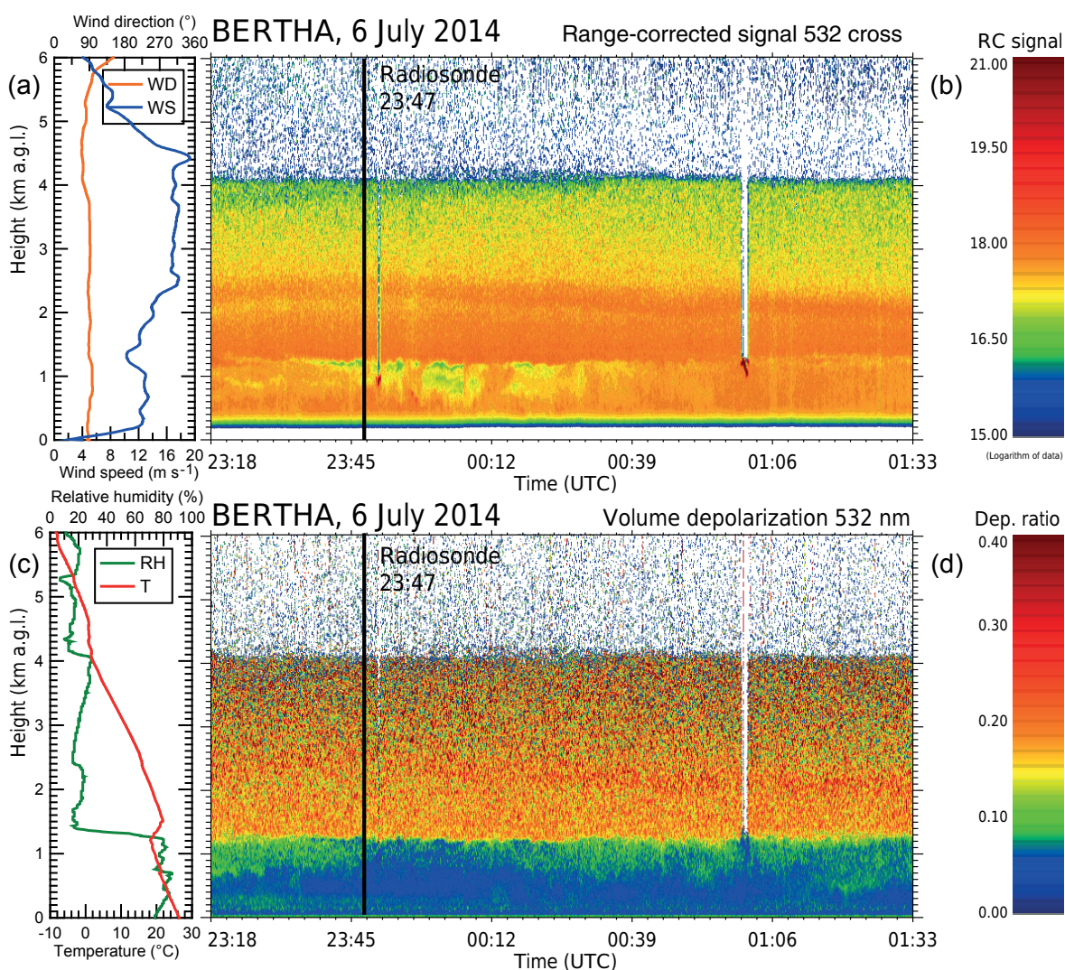
Figure 11. Saharan air layer (from 1.2 to 4.2 km height) above the marine boundary layer. The same parameters as in Fig. 2 are shown. The lidar observation was performed on 6 July 2014, 19:18–21:33 LT. The radiosonde was launched at 19:47 LT (indicated by a black vertical line).
